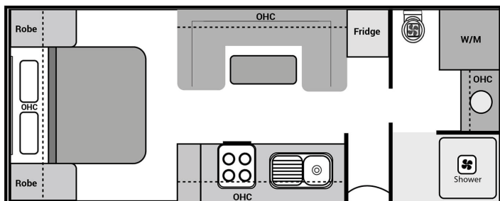
21'6 REAR DOOR CLUB LOUNGE
