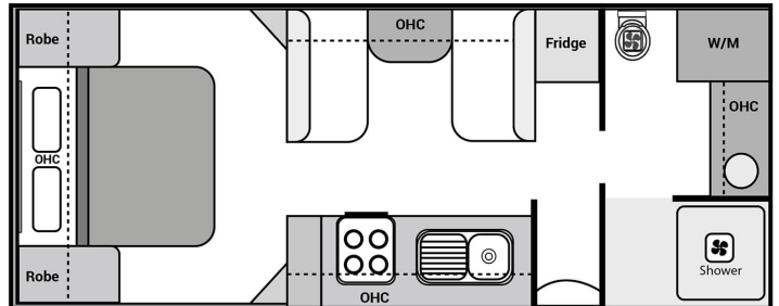
19'6 REAR DOOR CAFE DINETTE LOUNGE
